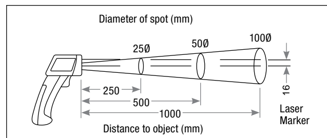
Spot size increases with distance from the probe tip as shown
